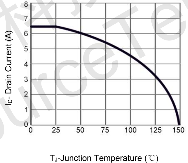
Figure 4 Drain Current
