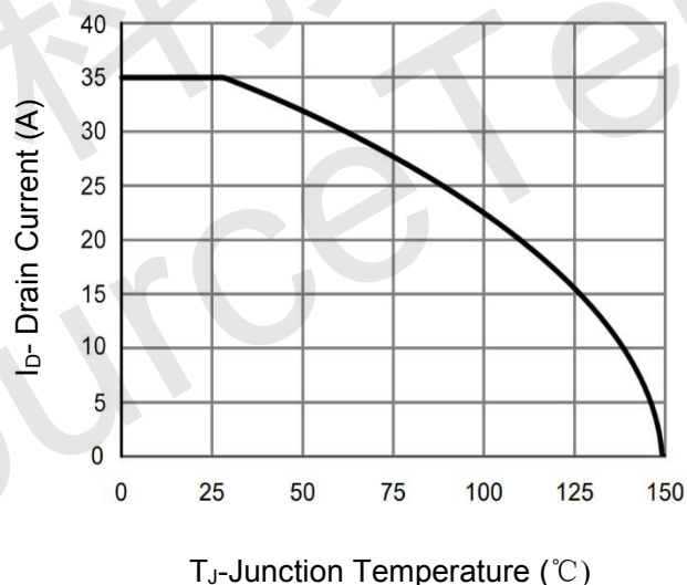
Figure 4 Drain Current
