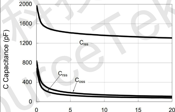
Figure 10 Capacitance vs Vds
