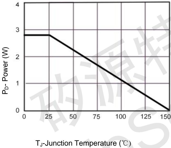
Figure 3 Power De-rating
