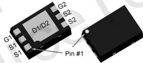
DFN2x3-6L
