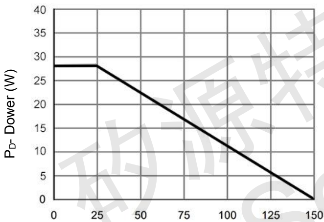
Figure 3 Power De-rating
