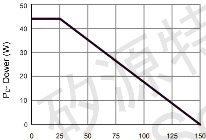
Figure 3 Power De-rating
