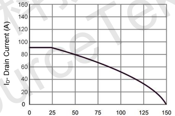
Figure 4 Drain Current
