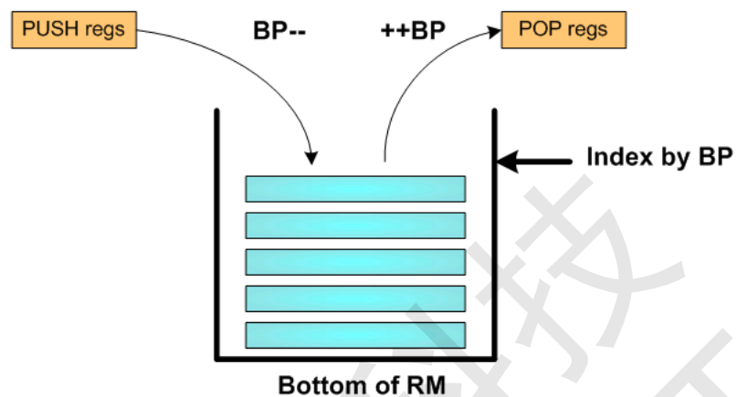
Figure 6.4 Data Stack Structure
