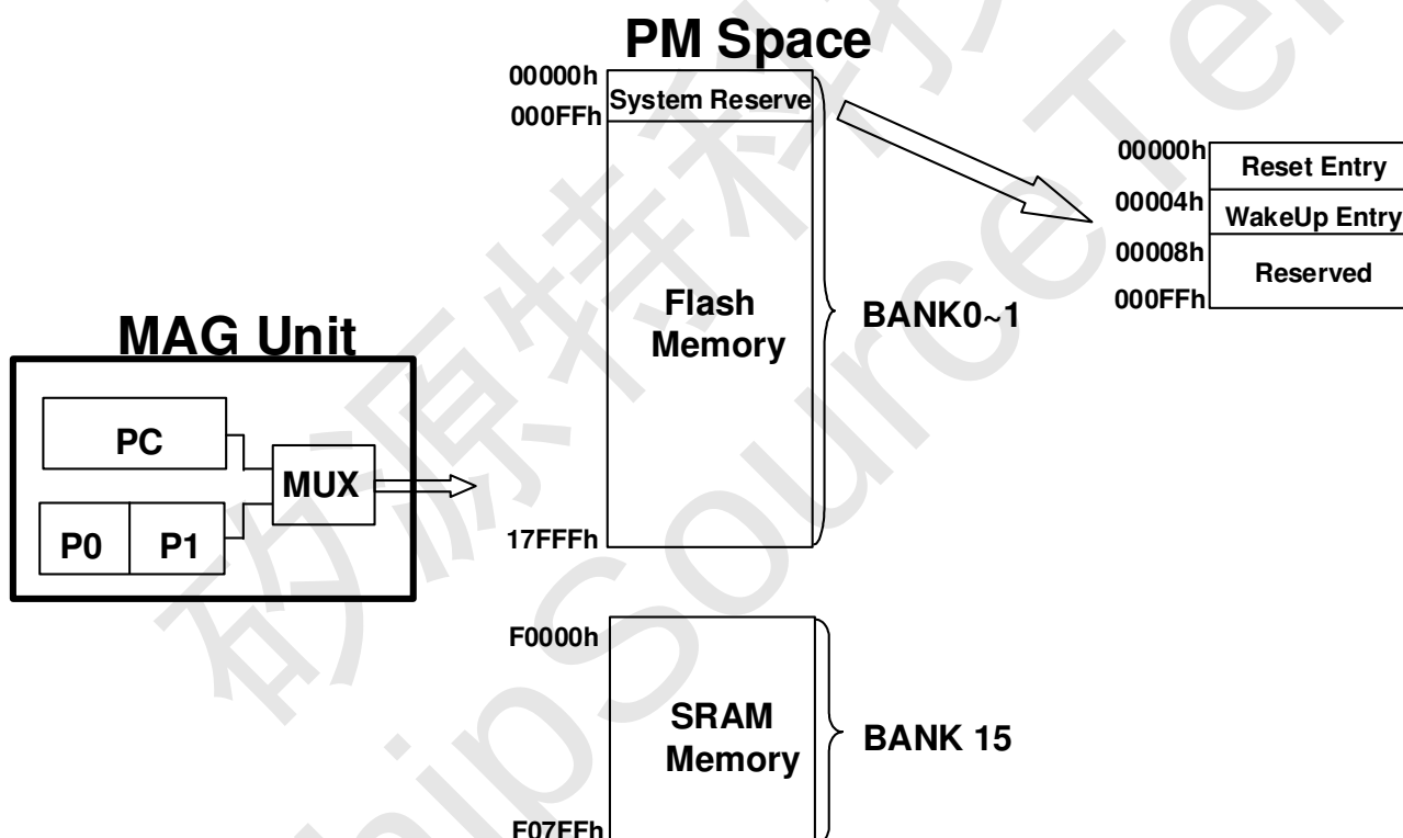
Figure 6.1 PM block diagram by DFFOFF instruction
