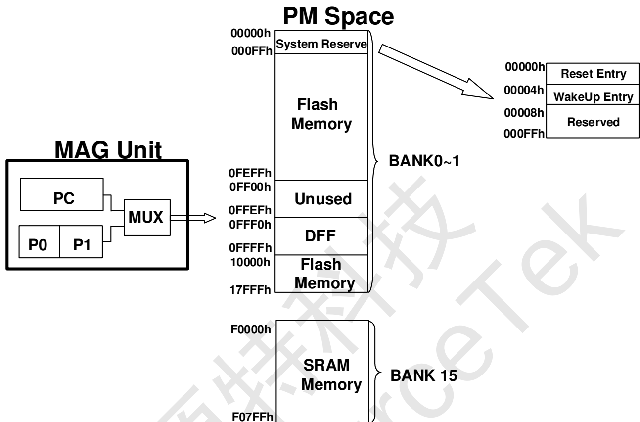
Figure 6.2 PM block diagram by DFFON instruction
