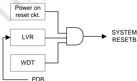
Figure 4 Reset structure
