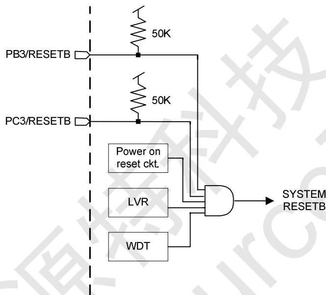
Figure 4 Reset structure
