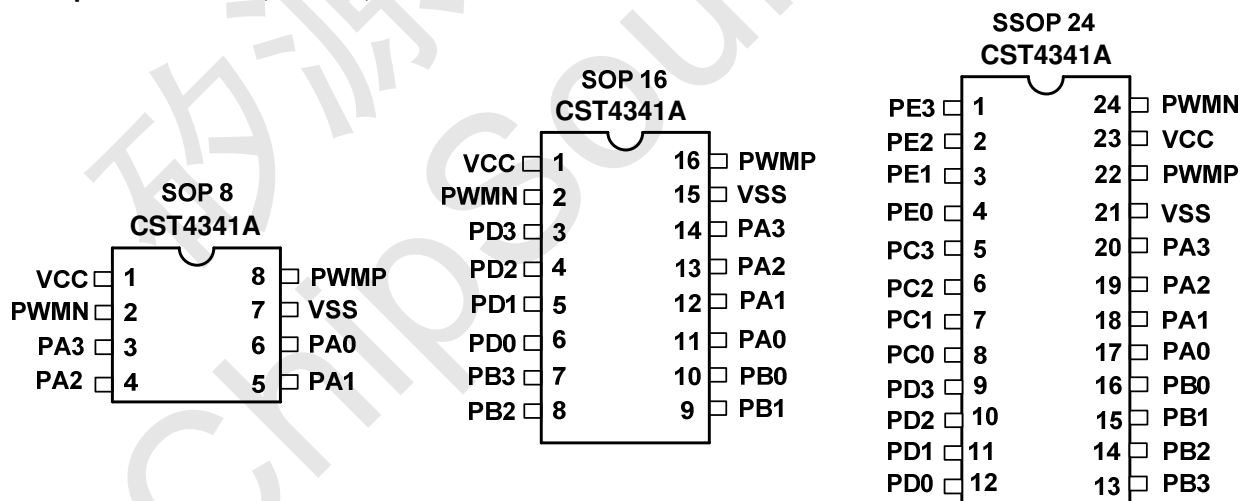
Figure1. Package definition
