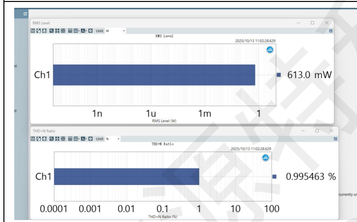
CST8302S 3.3V 8 欧 1%
