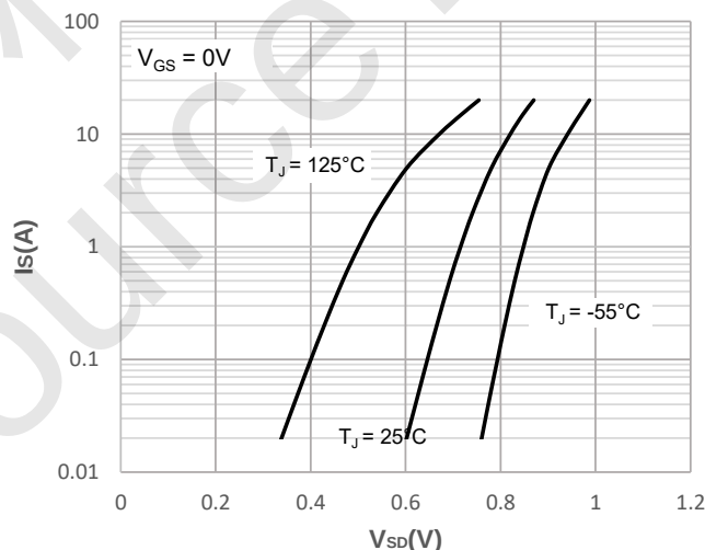
Figure 8: Body Diode Characteristics
