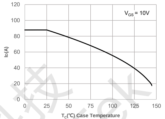
Figure 2: Current De-rating
