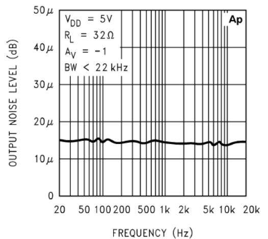
Noise Floor
