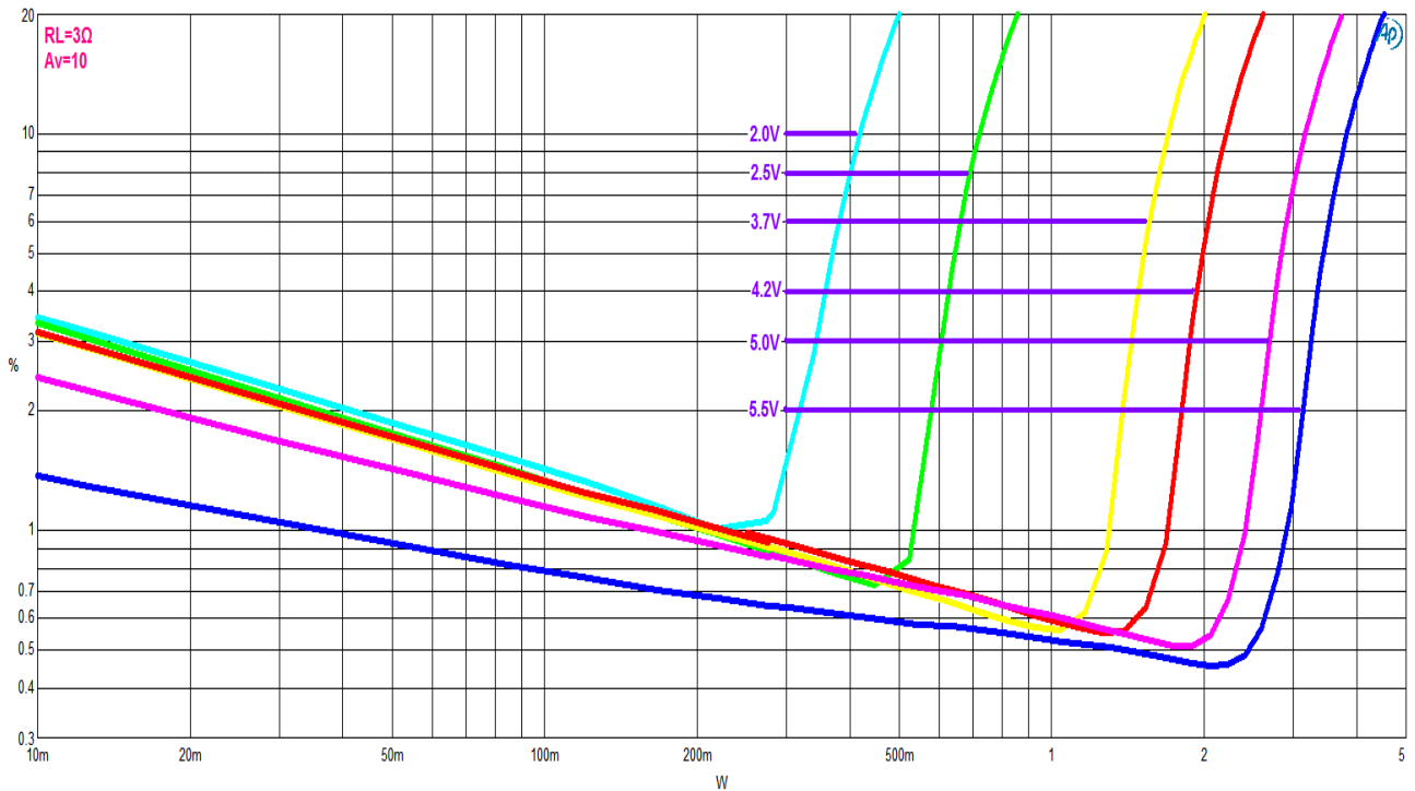
Figure 3 THD+N vs. Output Power (@ R_L=3\Omega , f=1\text{kHz} , A_v=10 )
