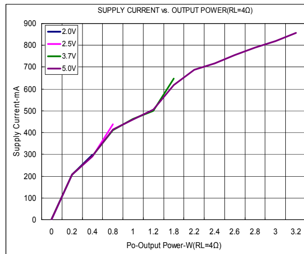
VDD Current vs. Output Power (RL=4Ω)
