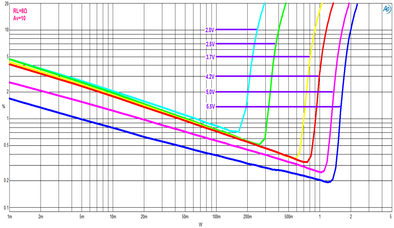
Figure 5 THD+N vs. Output Power (@ R_L=8\Omega , f=1\text{kHz} , A_v=10 )
