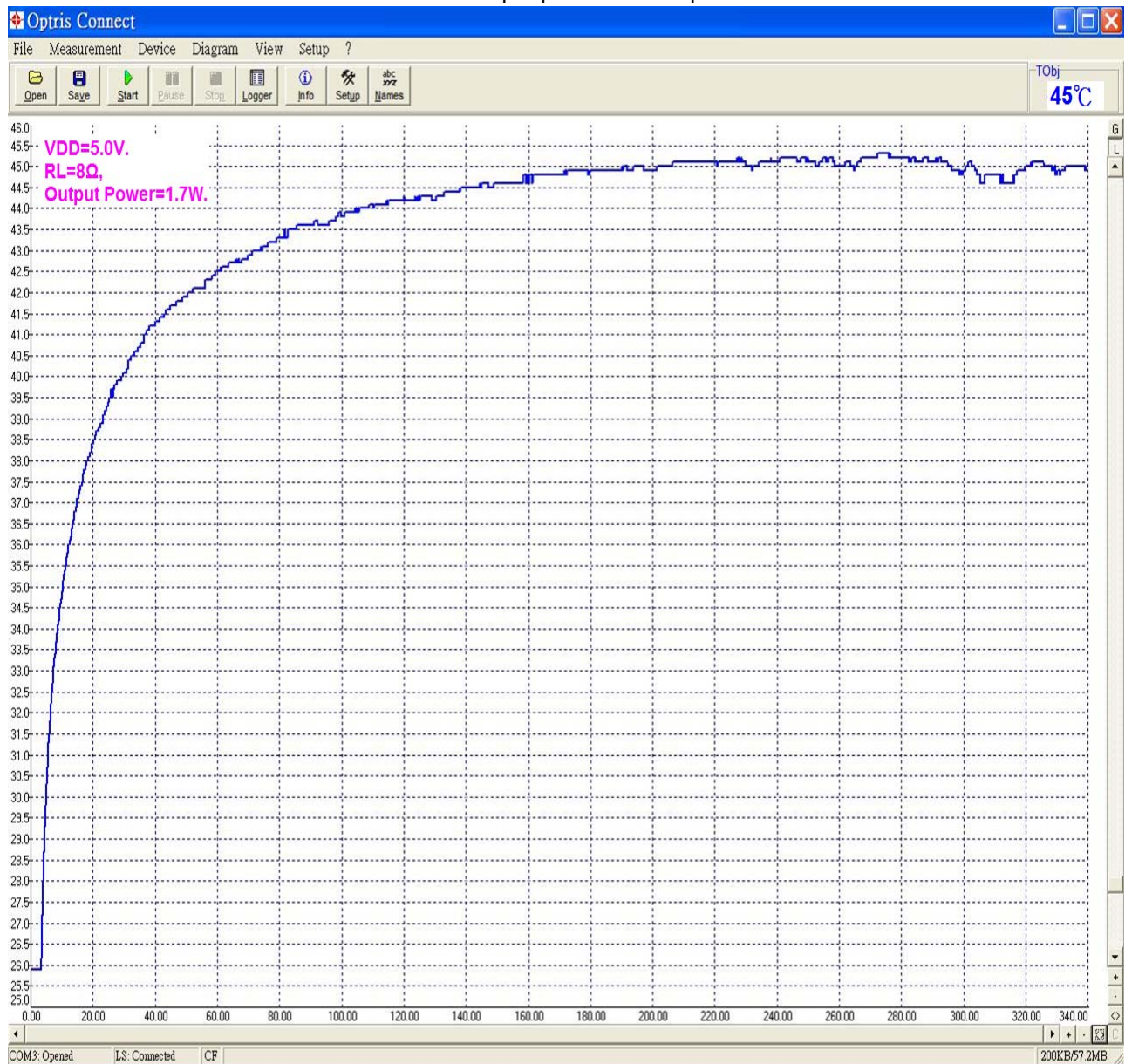
Output power vs. Temperature
