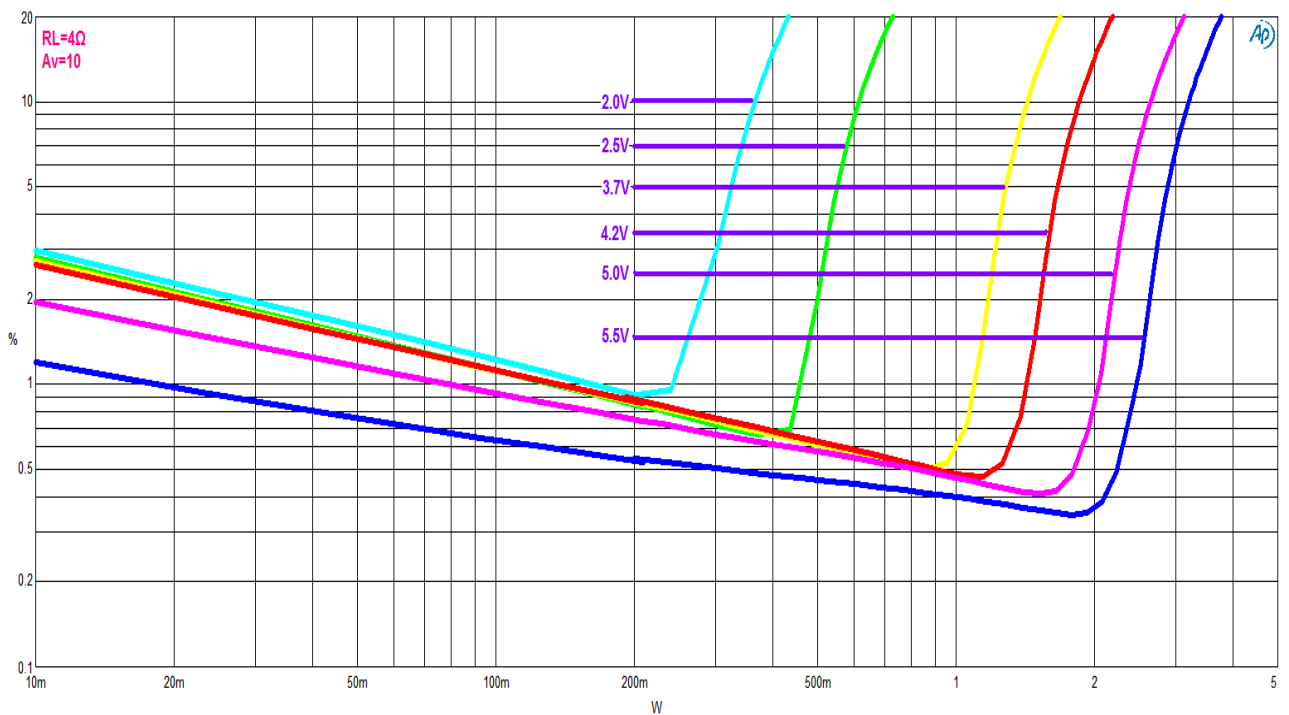
Figure 4 THD+N vs. Output Power (@ R_L=4\Omega , f=1\text{kHz} , A_v=10 )
