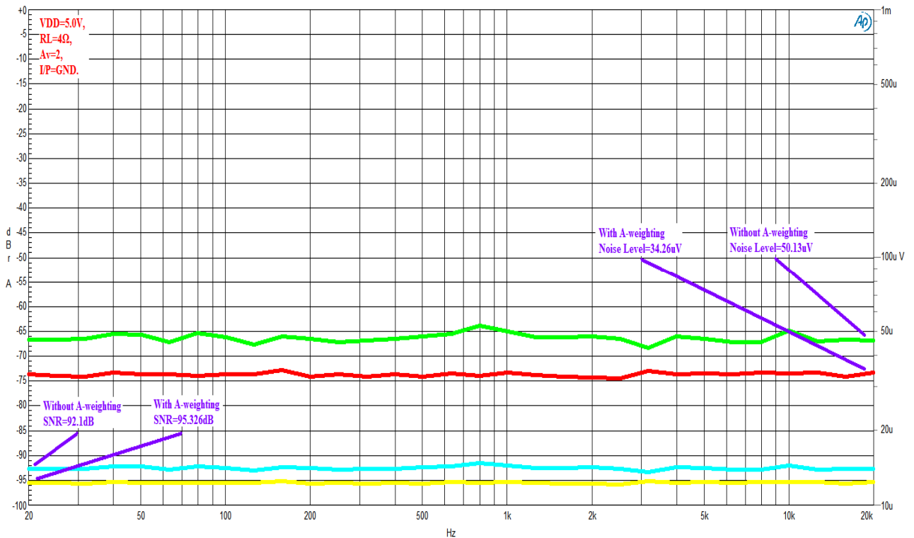
Figure 8 SNR vs. Noise Level
