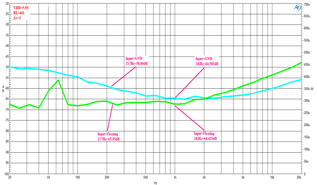
Figure 6 Power Supply Rejection Ratio (PSRR)
