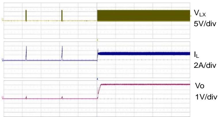
Fig.9 短路恢复 20ms/div
