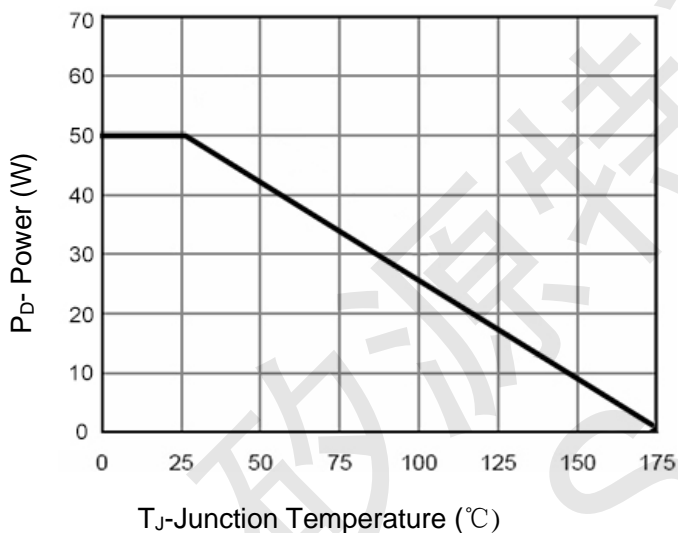
Figure 3 Power De-rating
