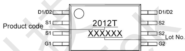
Marking and pin assignment
