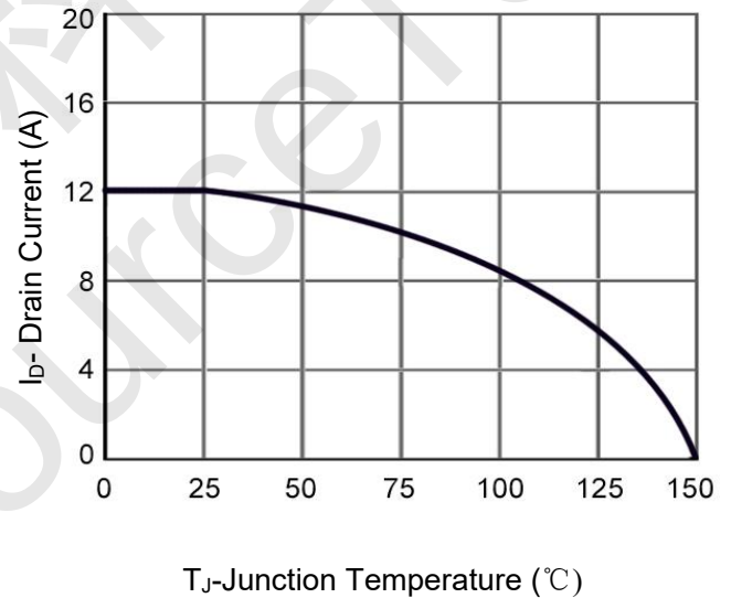
Figure 4 Drain Current
