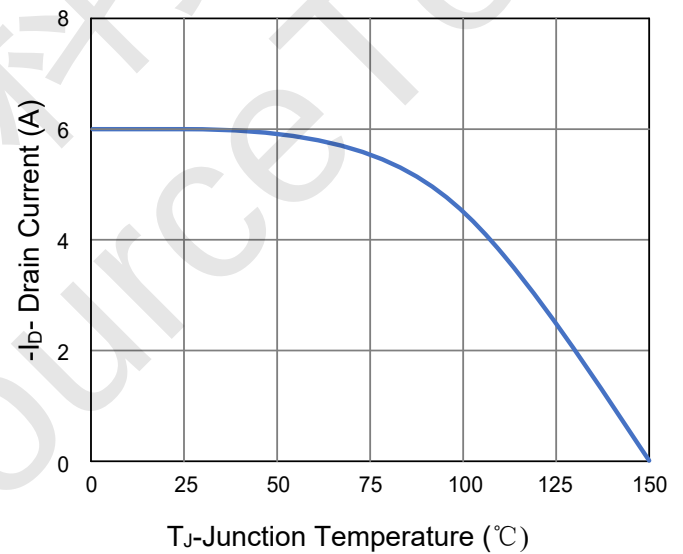
Figure 4 Drain Current
