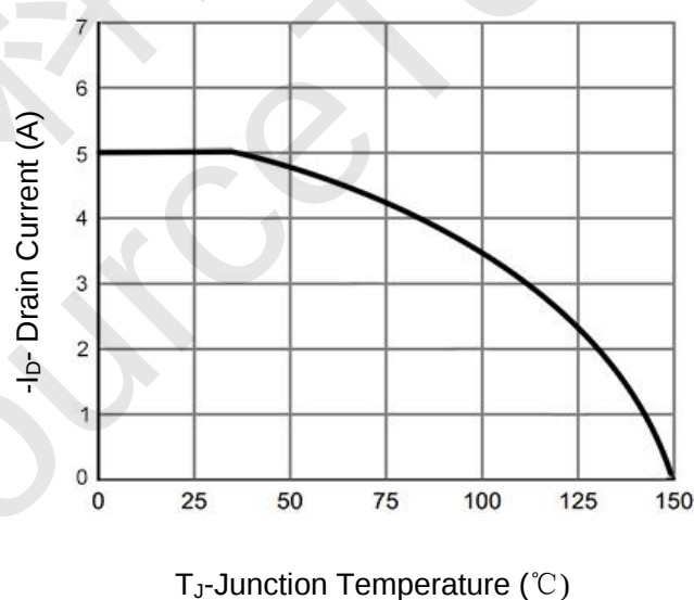
Figure 4 Drain Current
