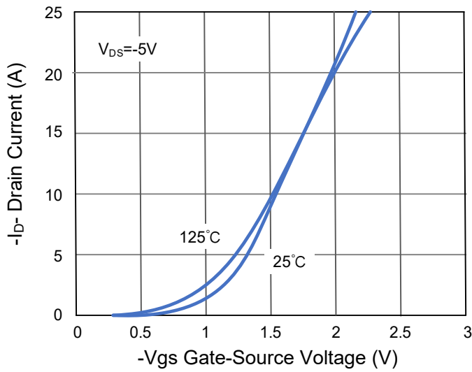
Figure 7 Transfer Characteristics
