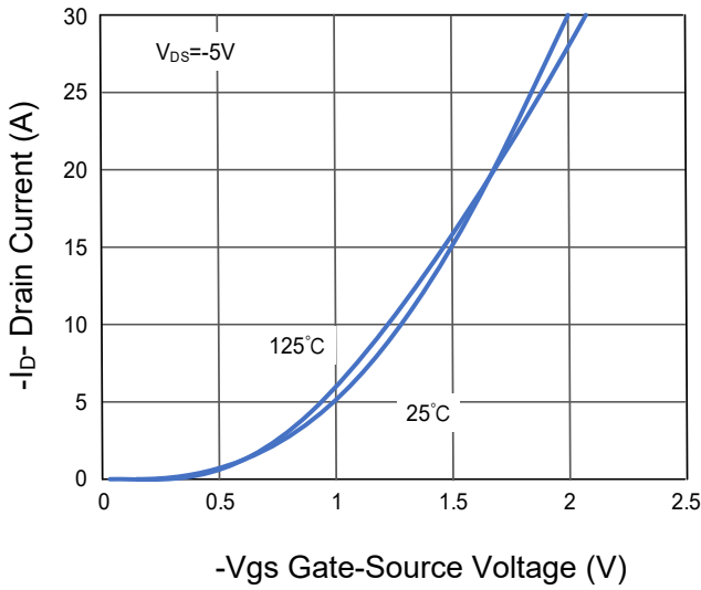
Figure 7 Transfer Characteristics
