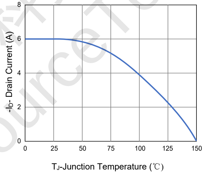
Figure 4 Drain Current
