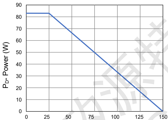
Figure 3 Power De-rating
