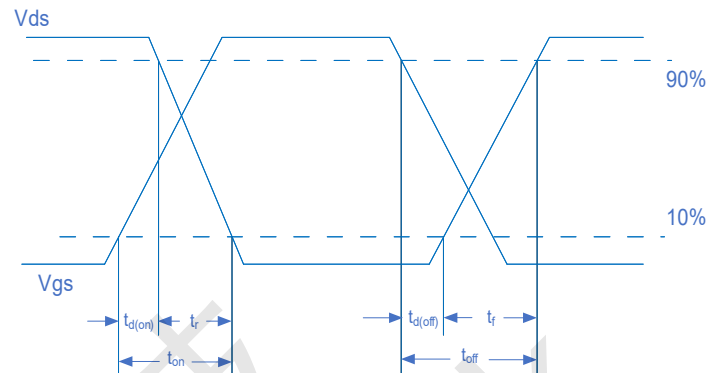
Figure 2 Switching Waveform
