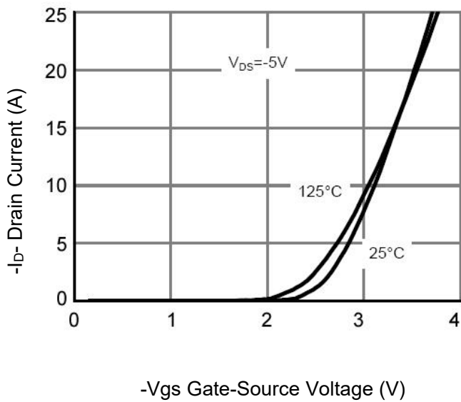
Figure 7 Transfer Characteristics
