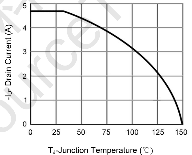
Figure 4 Drain Current
