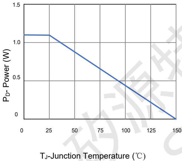
Figure 3 Power De-rating
