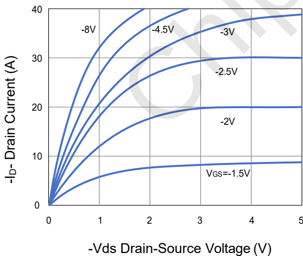
Figure 5 Output Characteristics
