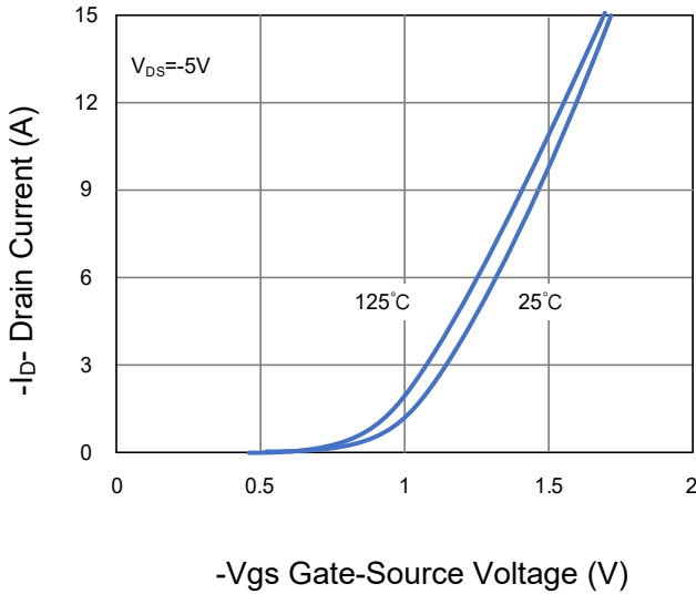
Figure 7 Transfer Characteristics
