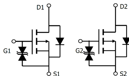
Schematic diagram
