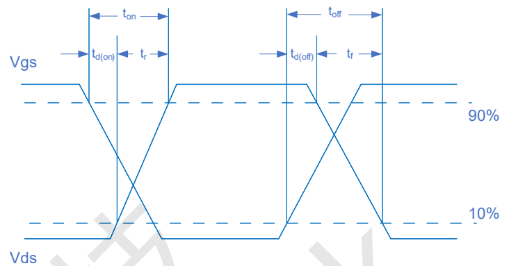
Figure 2 Switching Waveform
