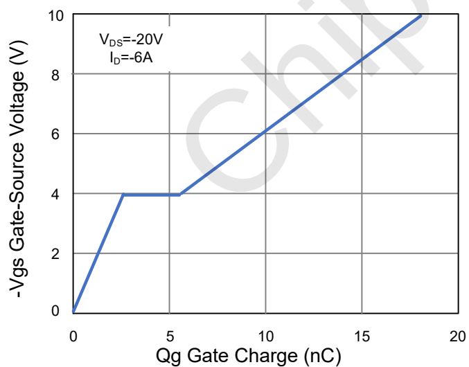
Figure 11 Gate Charge
