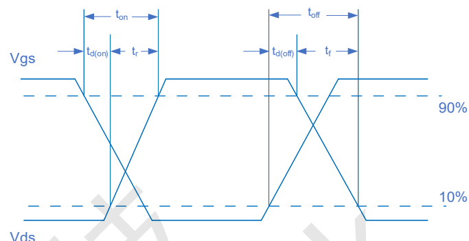
Figure 2 Switching Waveform
