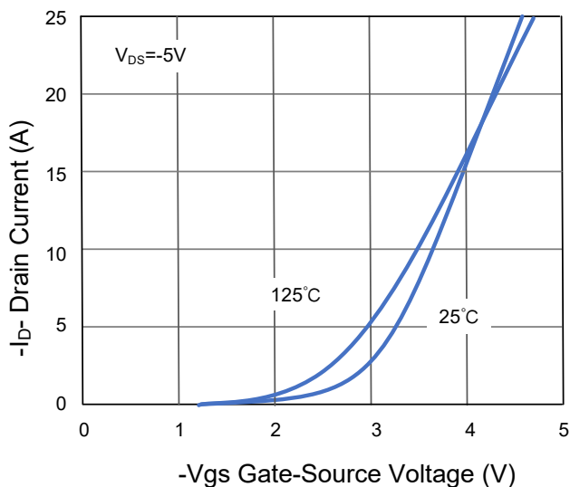
Figure 7 Transfer Characteristics
