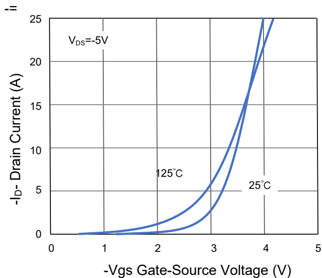
Figure 7 Transfer Characteristics
