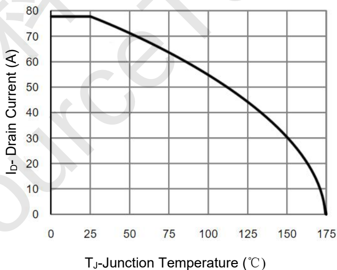
Figure 4 Drain Current
