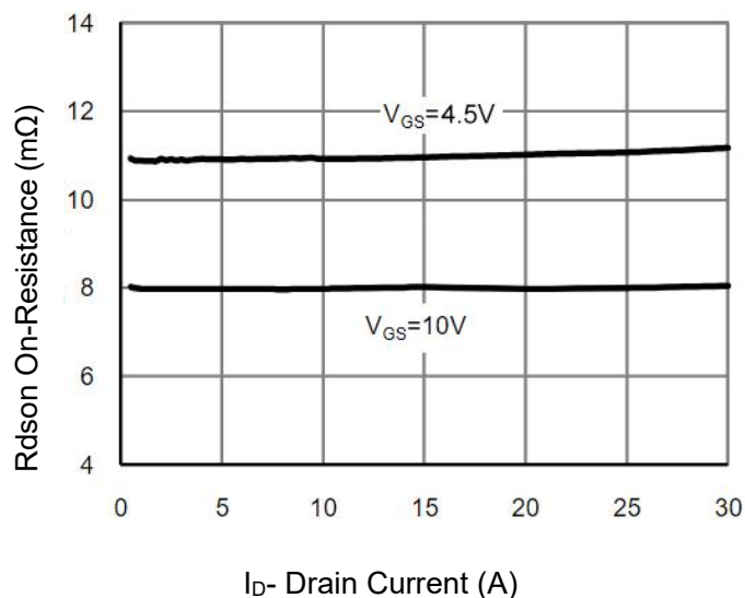
Figure 6 Rdson vs Drain Current
