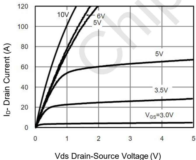
Figure 5 Output Characteristics
