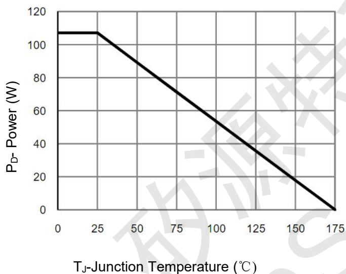
Figure 3 Power De-rating
