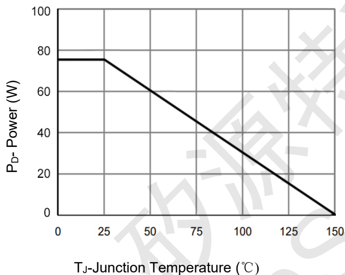
Figure 3 Power De-rating
