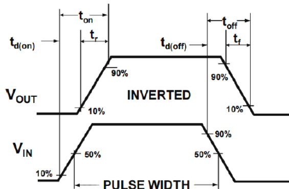
Figure 2 Switching Waveform
