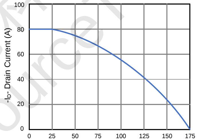
T J -Junction Temperature (°C)
