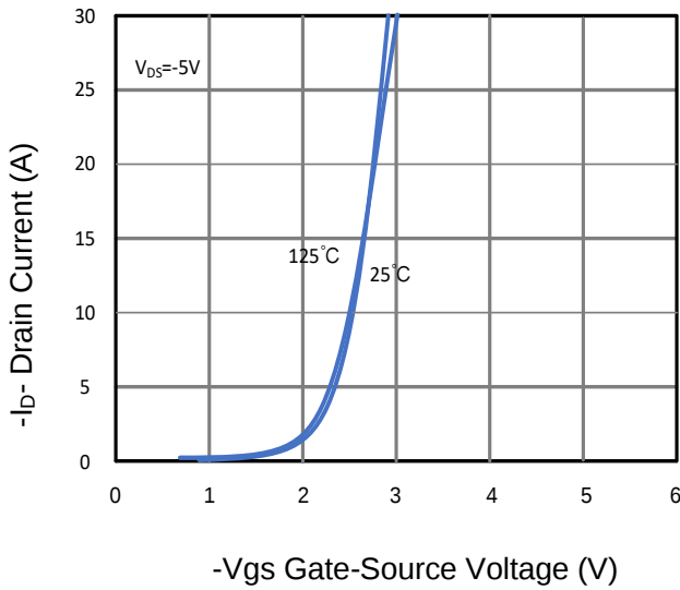
Figure 7 Transfer Characteristics
