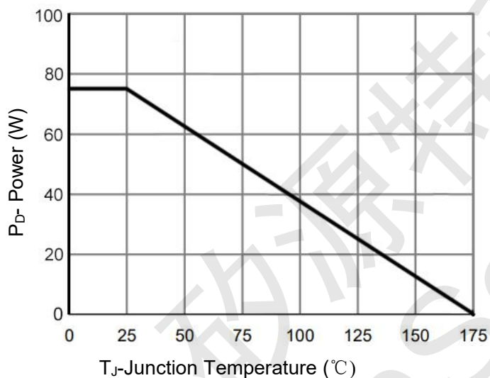
Figure 3 Power De-rating
