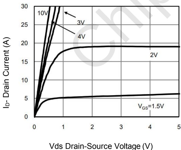
Figure 5 Output Characteristics
