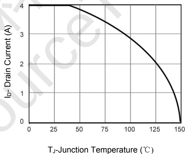
Figure 4 Drain Current
