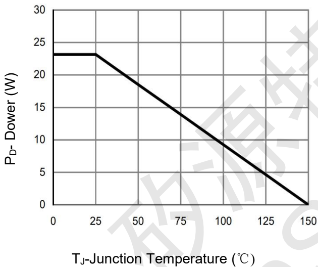
Figure 3 Power De-rating
