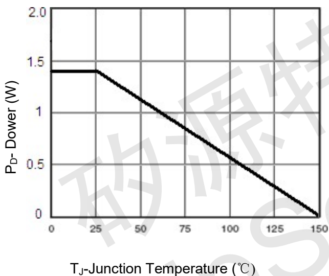
Figure 3 Power De-rating
