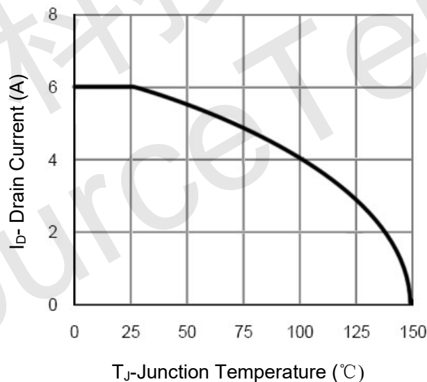
Figure 4 Drain Current
