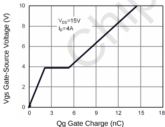
Figure 11 Gate Charge
