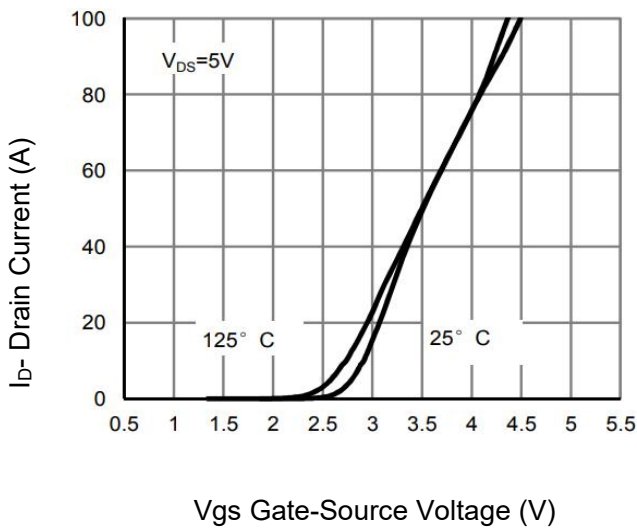
Figure 7 Transfer Characteristics
