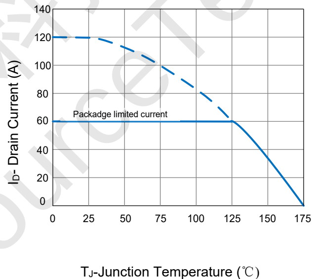
Figure 4 Drain Current
