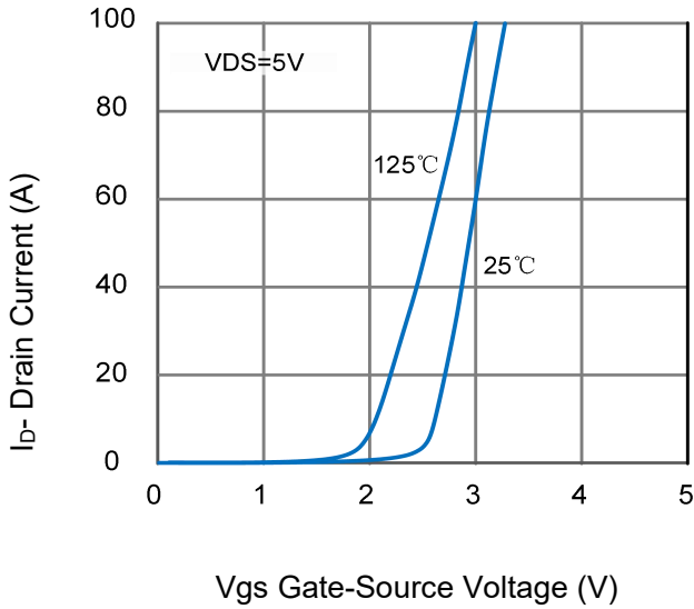
Figure 7 Transfer Characteristics
