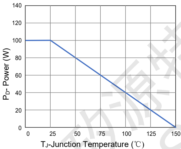
Figure 3 Power De-rating
