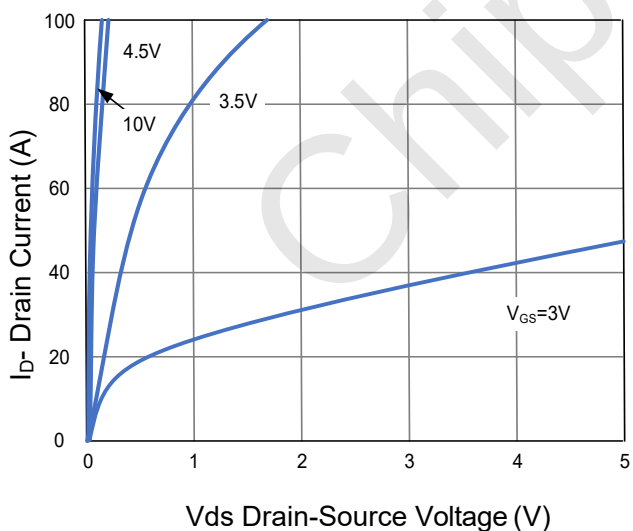
Figure 5 Output Characteristics
