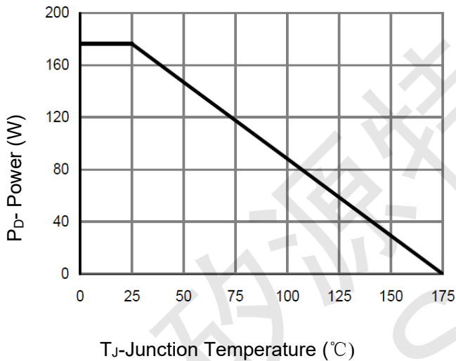
Figure 3 Power De-rating
