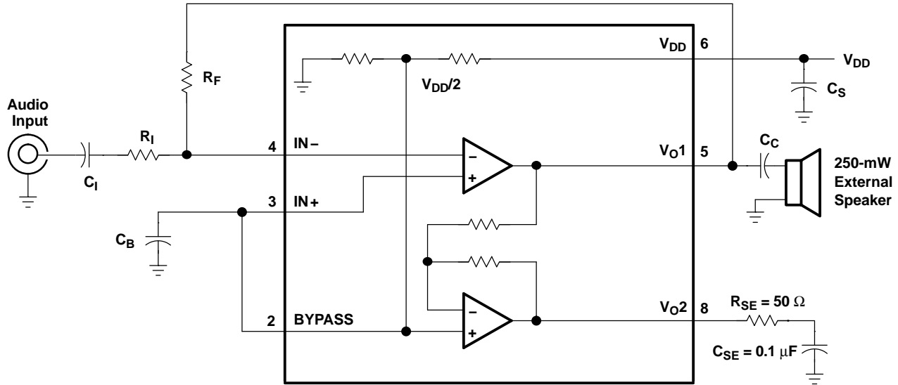
Figure 38. Singled-Ended Mode
