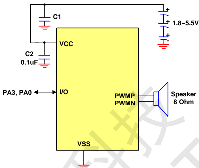
Figure 5. Applications circuit
