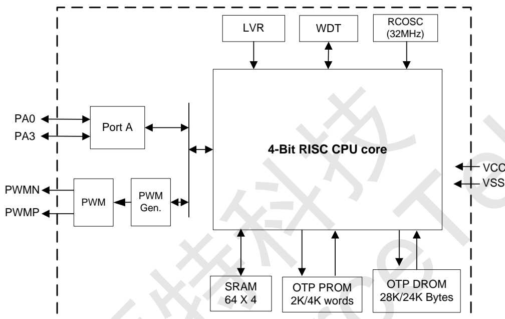
Figure 2. Block diagram
