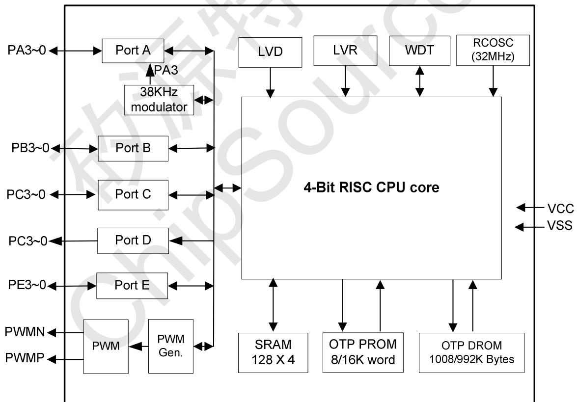
Figure 2. Block diagram
