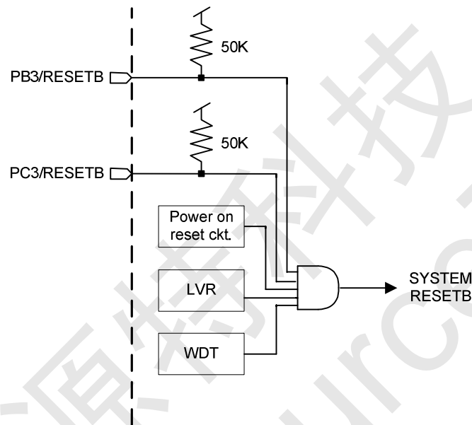
Figure 4 Reset structure
