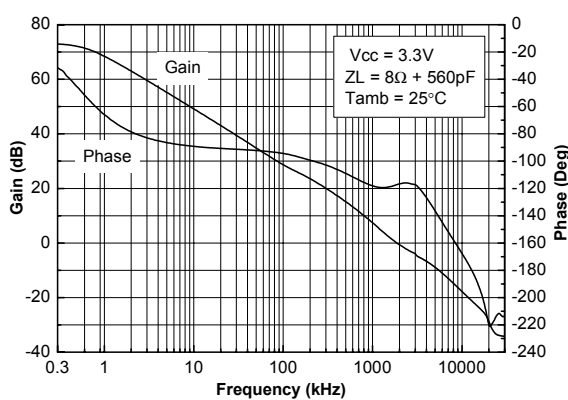
Figure 5. Open loop frequency response V_{CC}=3.3\text{ V} , Z_L=8\Omega
