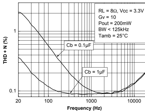
Figure 59. THD + N vs frequency, Pout=200 mW
