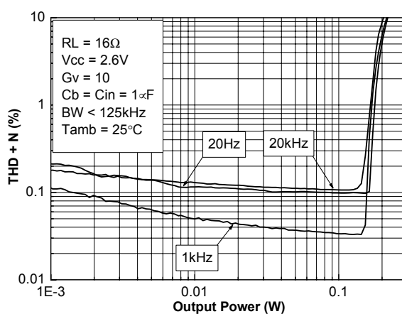
Figure 45. THD + N vs output power RL=16\ \Omega , V_{CC}=2.6\ V , G_v=10
