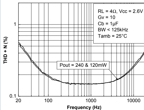
Figure 51. THD + N vs frequency, V_{CC}=2.6\text{ V} , RL = 4\Omega
