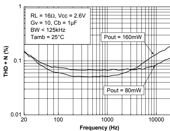
Figure 69. THD + N vs frequency, R_L=16\ \Omega , G_v=10 , P_{out}=160\ mW
