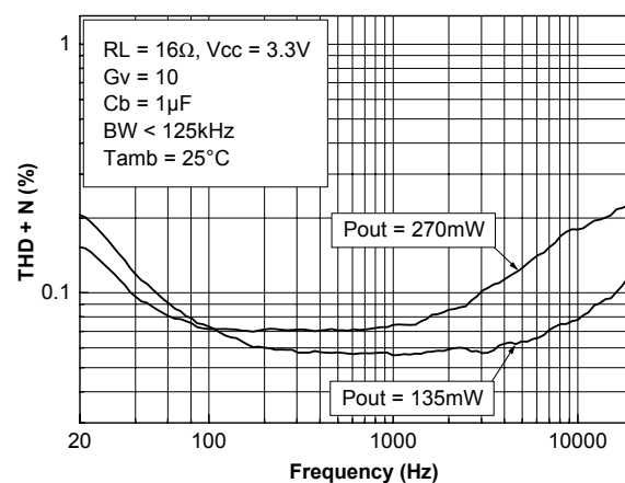
Figure 67. THD + N vs frequency, R_L=16\ \Omega , G_v=10 , V_{cc}=3.3\ V
