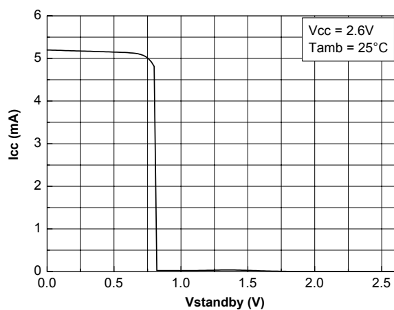
Figure 76. Current consumption vs standby voltage @ V cc = 2.6 V
