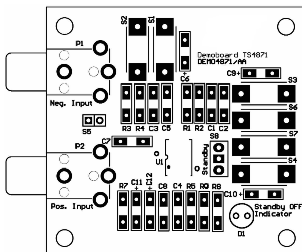
Figure 83. SO8 & MiniSO8 demoboard components side
