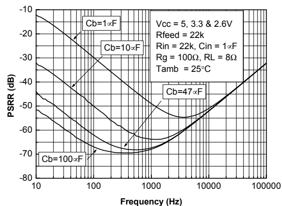
Figure 13. Power supply rejection ratio (PSRR) vs bypass capacitor
