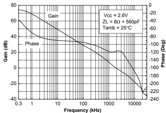
Figure 7. Open loop frequency response V_{CC}=2.6\text{ V} , Z_L=8\Omega
