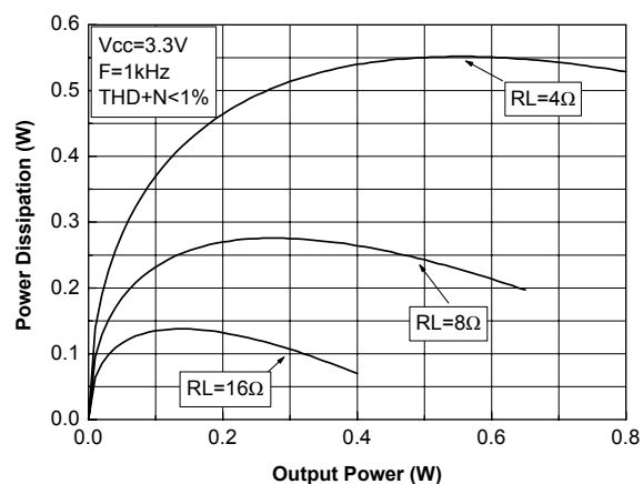
Figure 19. Power dissipation vs Pout Vcc=3.3 V
