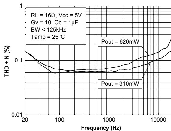
Figure 65. THD + N vs frequency, RL=16 Ω , Gv=10
