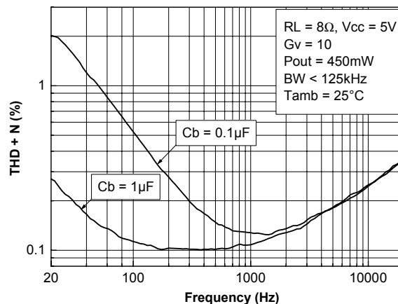
Figure 55. THD + N vs frequency, Pout=450 mW, RL=8 Ω
