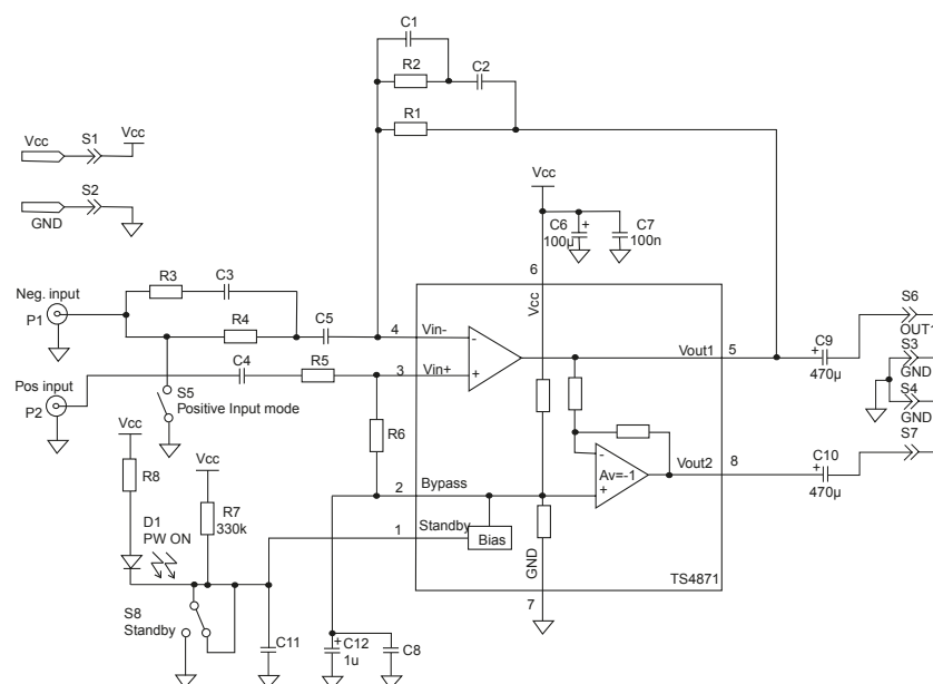
Figure 82. Demoboard schematic
