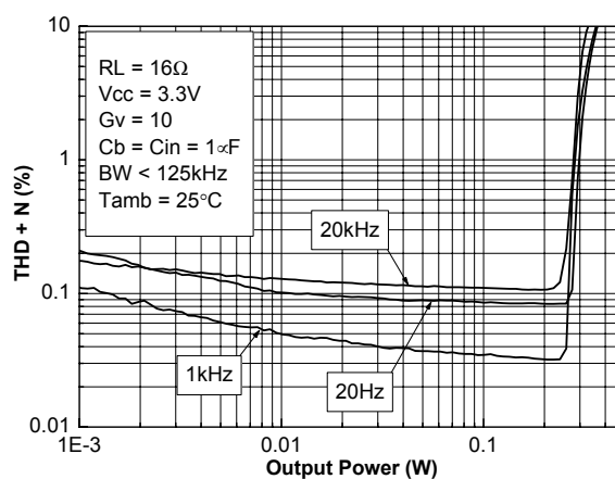
Figure 43. THD + N vs output power RL=16\ \Omega , G_v=10 , V_{CC}=3.3\ V
