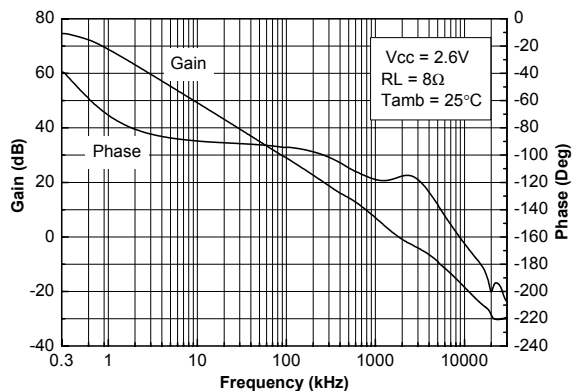
Figure 6. Open loop frequency response V_{CC}=2.6\text{ V}
