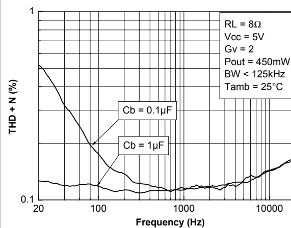
Figure 53. THD + N vs frequency, P_{out}=450\text{ mW}
