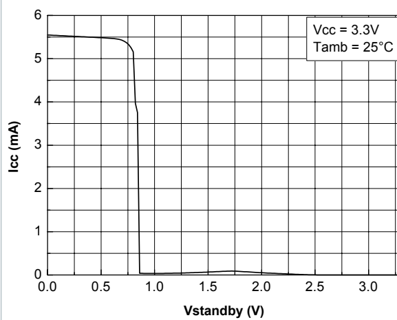
Figure 77. Current consumption vs standby voltage @ V cc = 3.3 V
