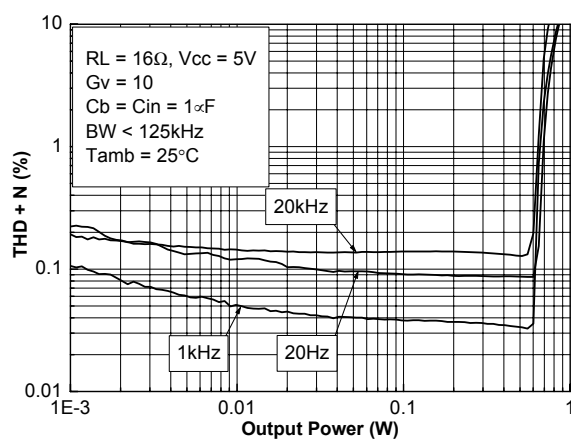
Figure 41. THD + N vs output power RL=16\text{ }\Omega G_v=10
