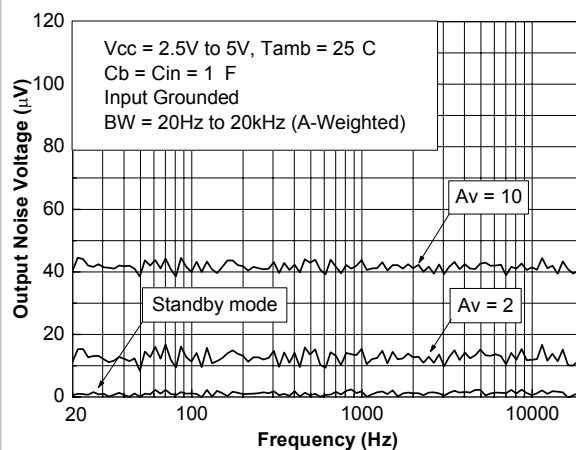
Figure 81. Vout1+Vout2 A-weighted noise floor
