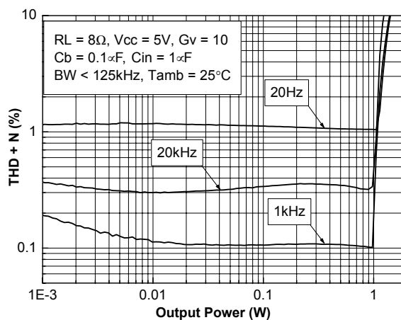
Figure 35. THD + N vs output power G_v=10 , V_{cc} = 5 V, C_b=0.1 \mu F
