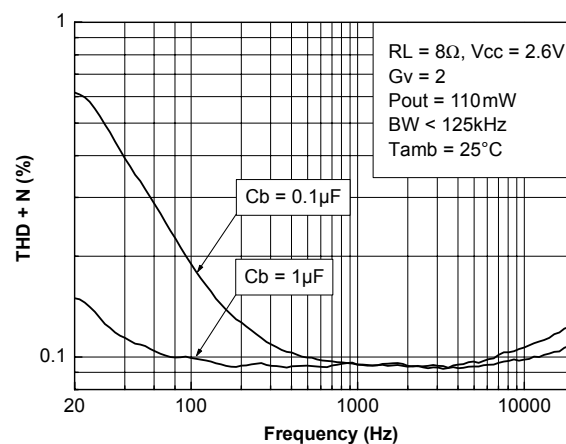
Figure 61. THD + N vs frequency, Pout=110 mW
