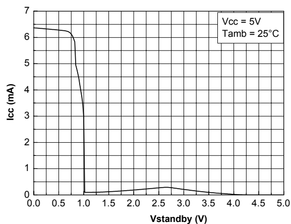
Figure 75. Current consumption vs standby voltage @ V cc = 5 V
