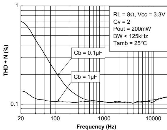
Figure 57. THD + N vs frequency, Pout=200 mW
