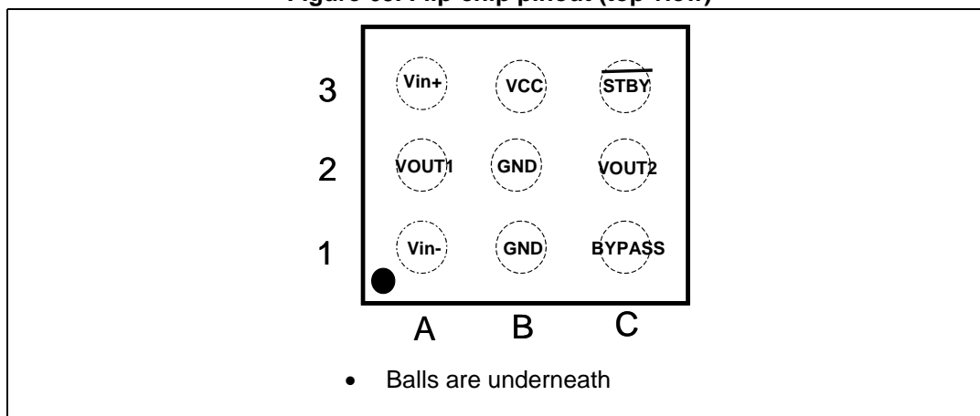
Figure 65. Flip-chip pinout (top view)
