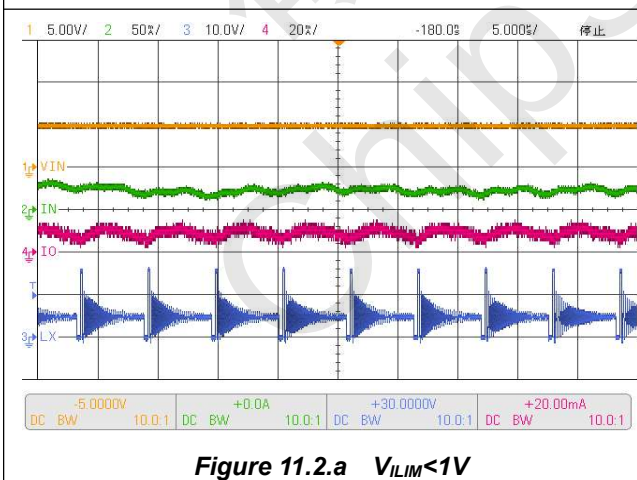
Figure 11.2 自适应限流
