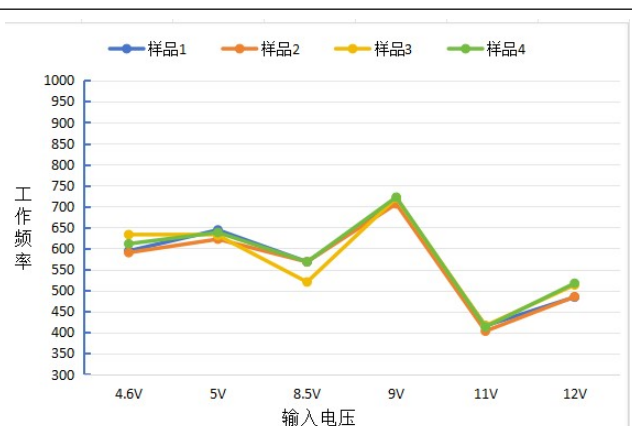
Figure 11.3 输入电压与开关频率
