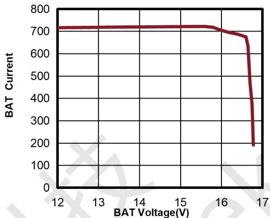
Figure 10.1.b R_{ICHG}=1.3K , 恒流和恒压充电电流
