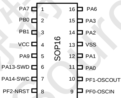
图 3-3 SOP16 Pinout1 ZH32F002AW15S
