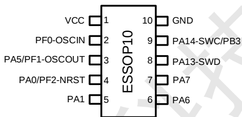
图 3-2 ESSOP10 Pinout1 ZH32F002AA15M
