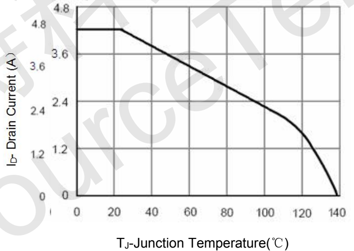
Figure 4 Drain Current
