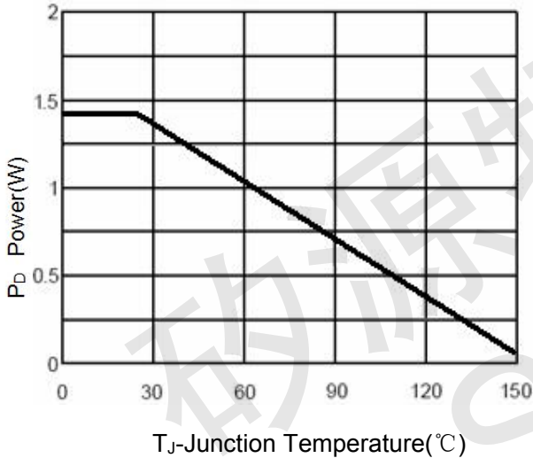
Figure 3 Power Dissipation
