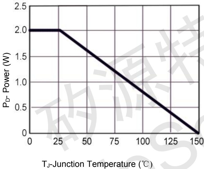
Figure 3 Power De-rating
